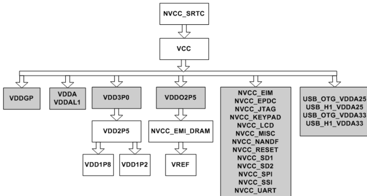
Figure 2. Power-Up Sequence
