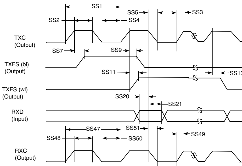
Figure 52. SSI Receiver Internal Clock Timing Diagram
