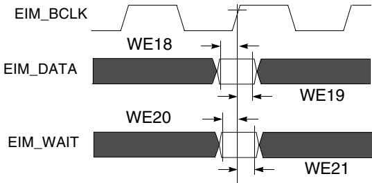
Figure 18. EIM Inputs Timing Diagram
