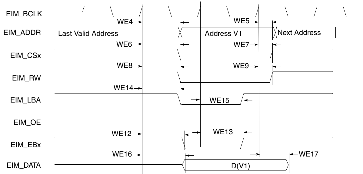
Figure 20. Synchronous Memory, Write Access, WSC=1, WBEA=1, WBEN=1, and WADV=0
