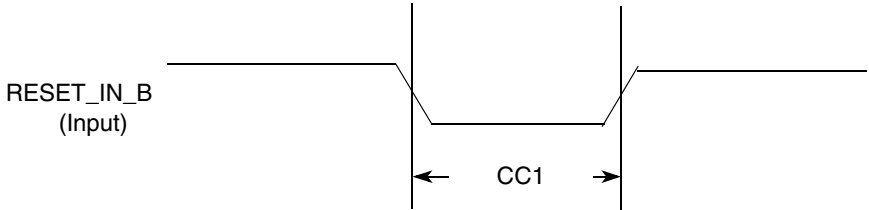
Figure 6. Reset Timing Diagram
