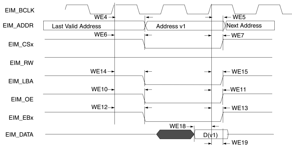
Figure 19. Synchronous Memory Read Access, WSC=1
