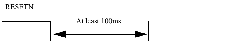
Figure 2. RESETN Timing
