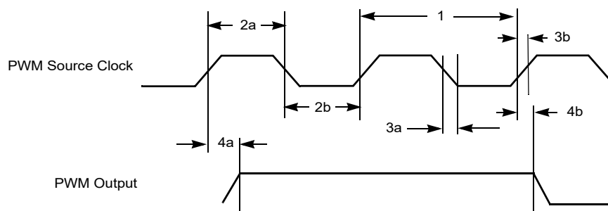
Figure 31. PWM Timing
