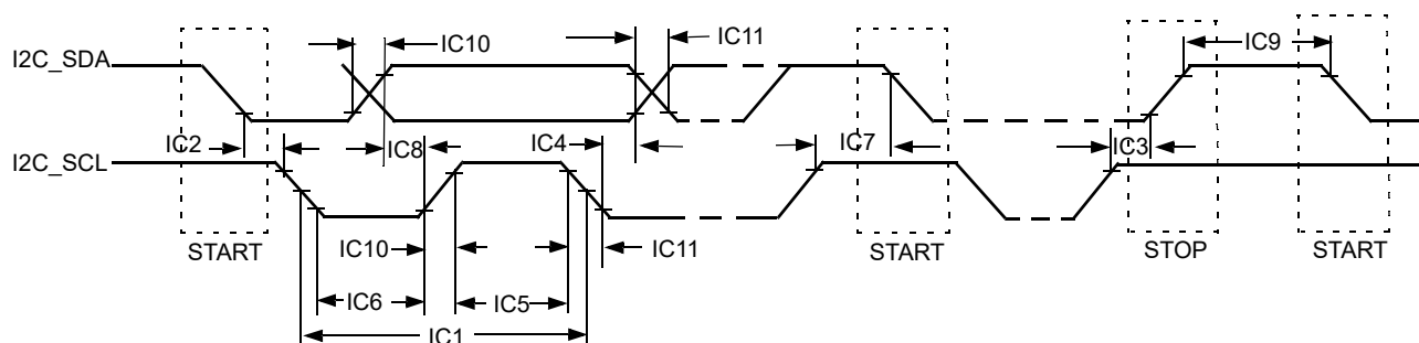
Figure 25. I 2 C Module Timing Diagram
