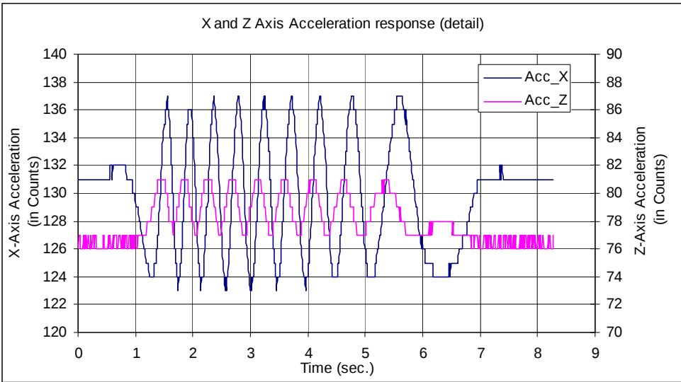
Figure 3-10. X- and Z-axis response with speed in the range of 1 to 2 ms -1
