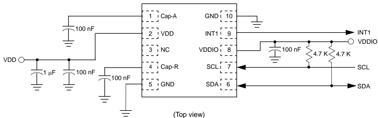
Figure 3. Electrical connection
