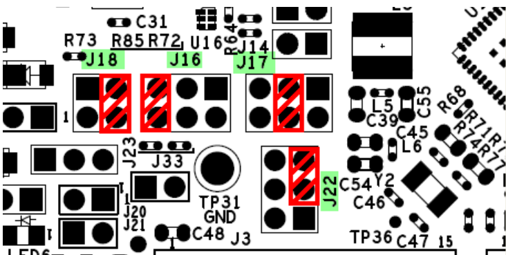
Figure 12. Buck headers
