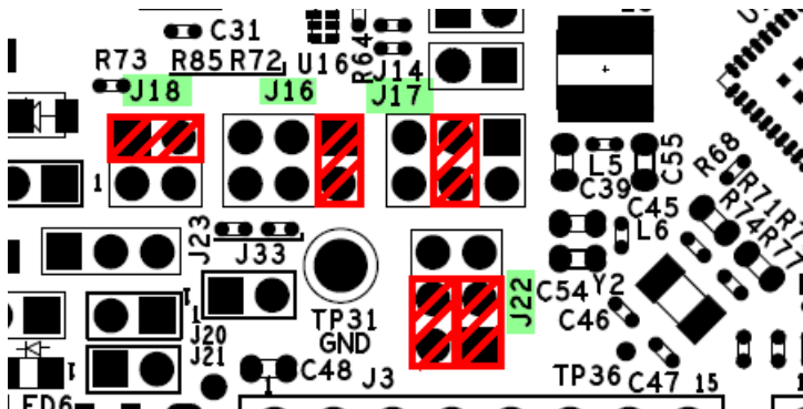
Figure 11. Bypass headers
