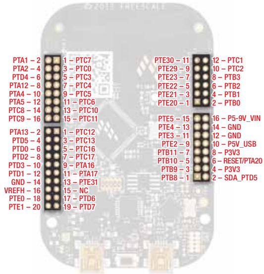
Figure 2: FRDM-KL25Z Pin-Out
