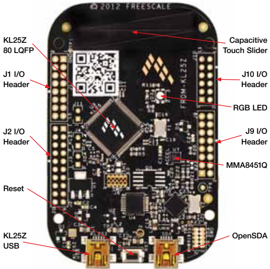
Figure 1: FRDM-KL25Z Callouts
