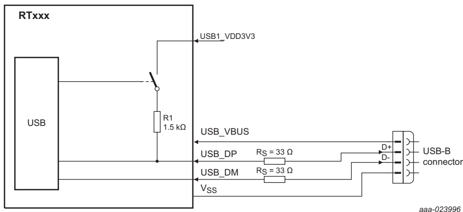
Fig 36. USB interface on a self-powered device where USB_VBUS = 5 V
