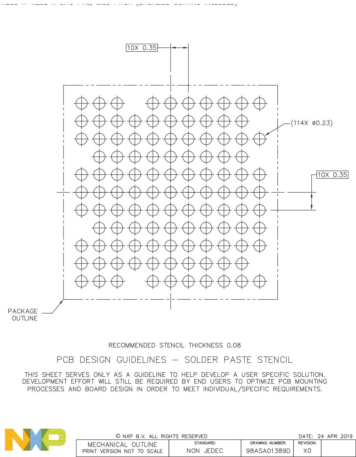
Fig 52. Reflow soldering of the WLCSP114 package (part 3 of 4)
