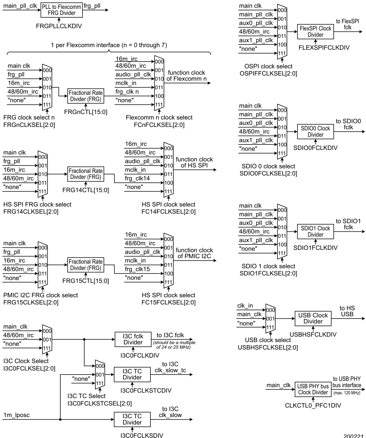
Fig 7. RT600 clock generation (continued)
