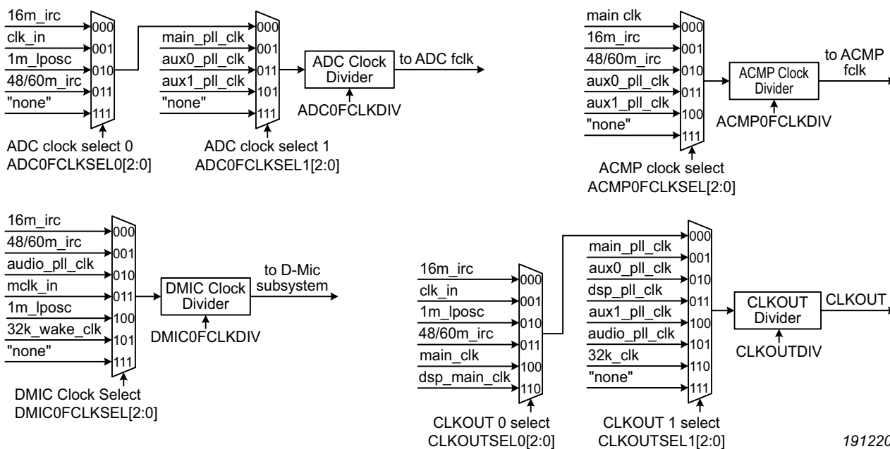
Fig 8. RT600 clock generation (continued)
