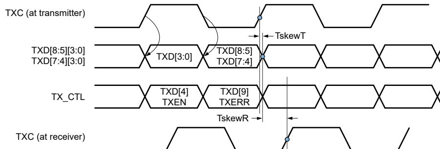
Figure 57. RGMII Transmit Timing
