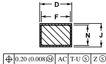
SECTION AE-AE
