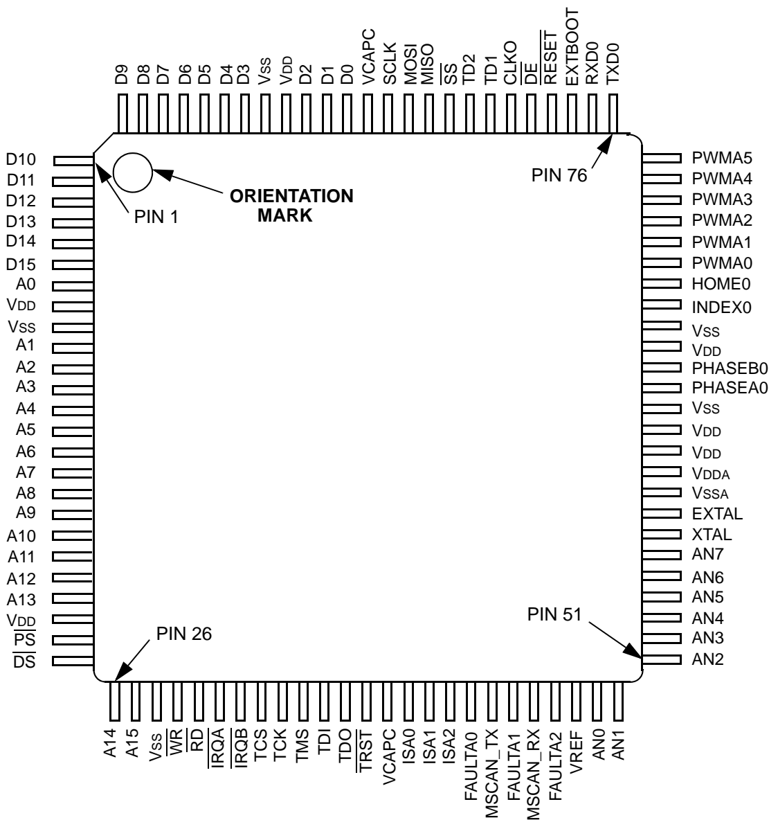
Figure 4-1 Top View, 56F803 100-pin LQFP Package
