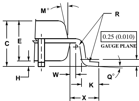
DETAIL AD
