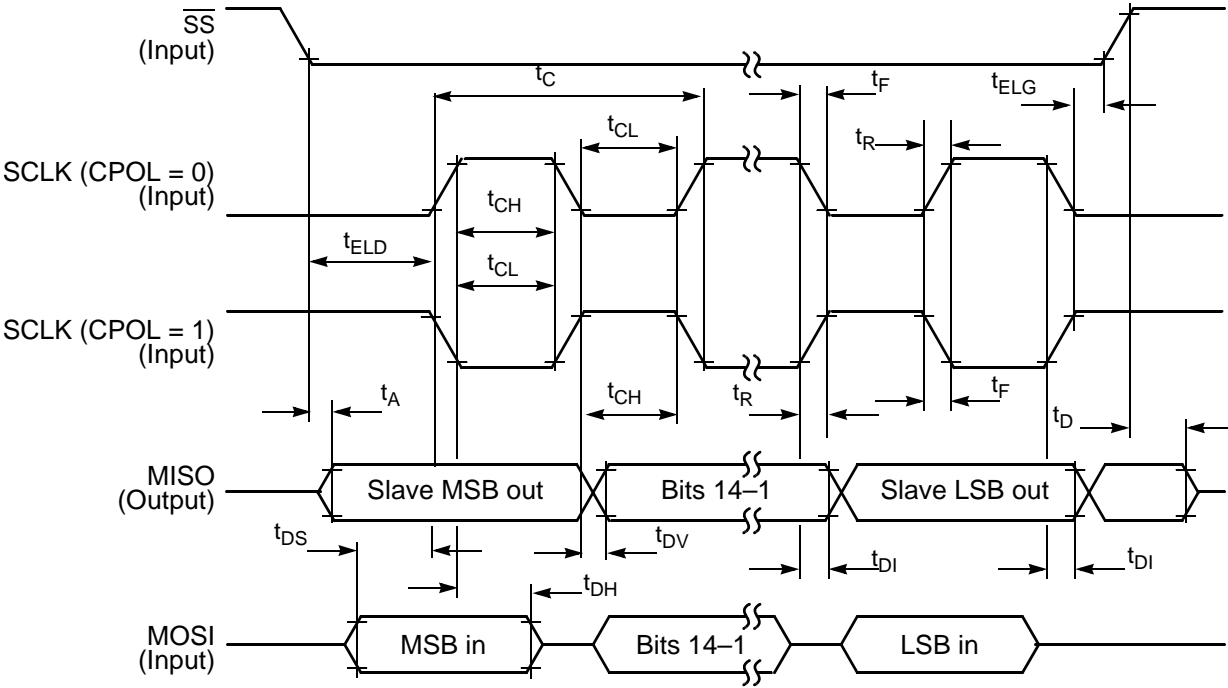
Figure 3-20 SPI Slave Timing (CPHA = 0)
