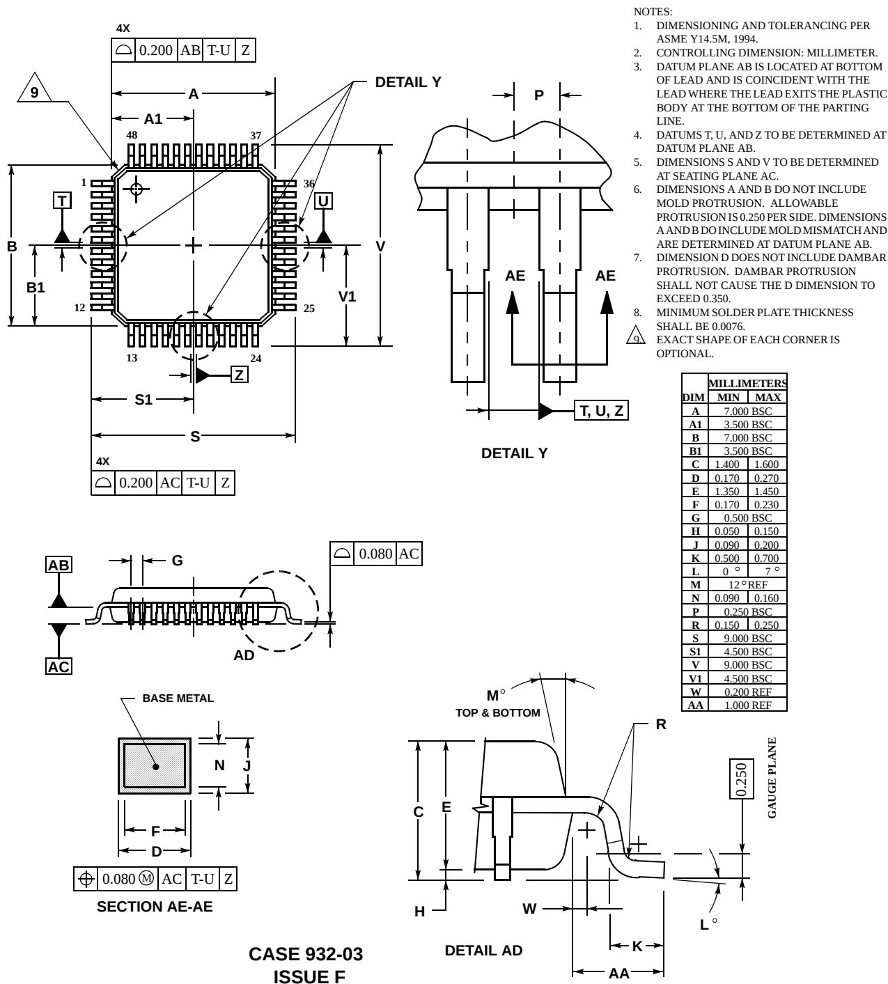
Figure 4-2 48-pin LQFP Mechanical Information
