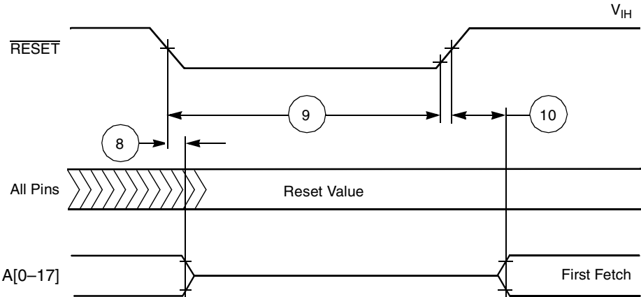
Figure 2-3. Reset Timing
