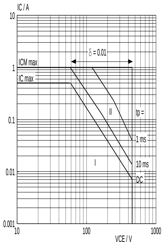
Fig.10. Forward bias safe operating area. T_{mb} = 25\text{ }^{\circ}\text{C}
