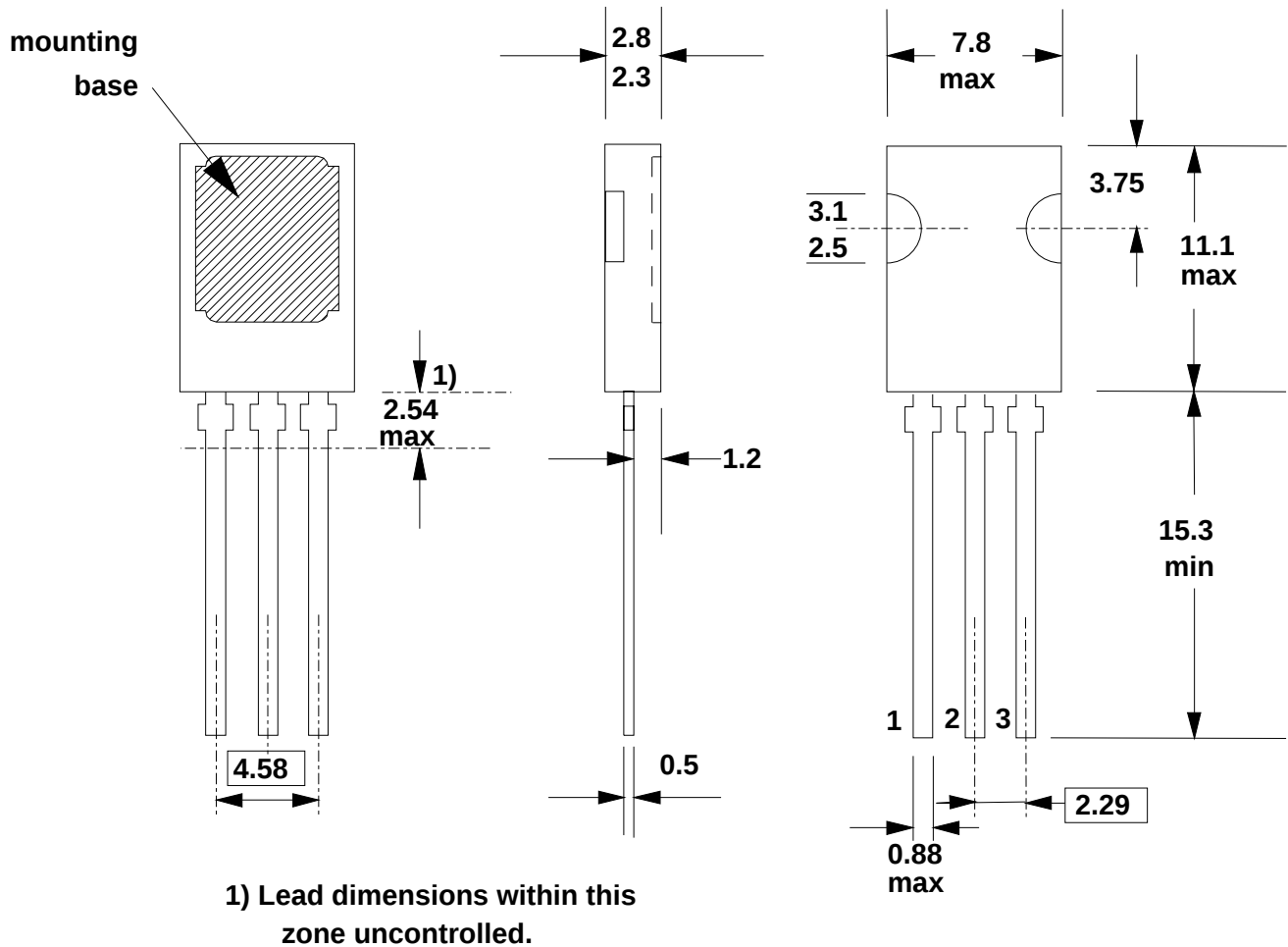
Fig.11. SOT82; pin 2 connected to mounting base.
