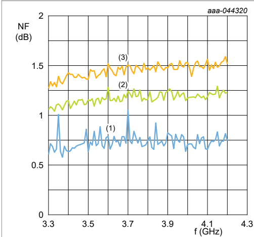
Figure 8. High gain RX mode, NF versus frequency over temperature (1) T_{case} = -40\text{ }^{\circ}\text{C} (2) T_{case} = 50\text{ }^{\circ}\text{C} (3) T_{case} = 105\text{ }^{\circ}\text{C}
