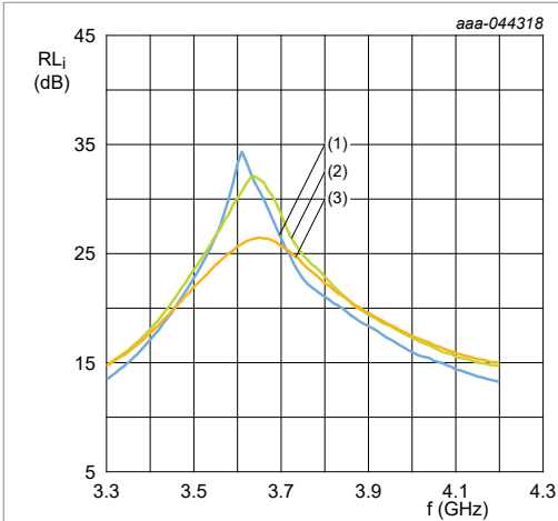
Figure 6. High gain RX mode, RL_i versus frequency over temperature (1) T_{case} = -40\text{ }^{\circ}\text{C} (2) T_{case} = 50\text{ }^{\circ}\text{C} (3) T_{case} = 105\text{ }^{\circ}\text{C}
