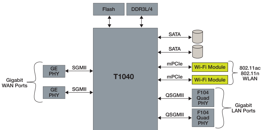
Figure 1. Security Appliance/UTM Equipment Block Diagram
