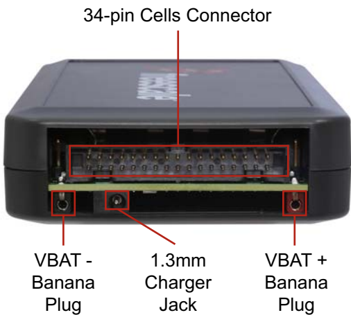
Figure 4. Side View
