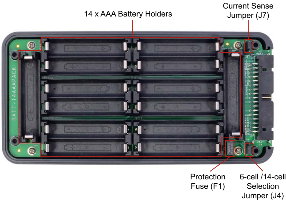
Figure 3. Top View
