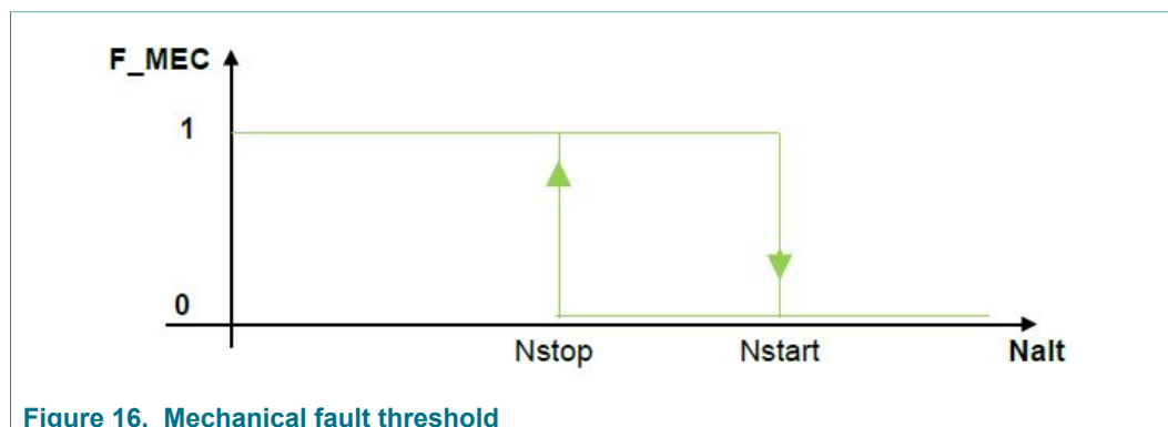
Figure 16. Mechanical fault threshold
