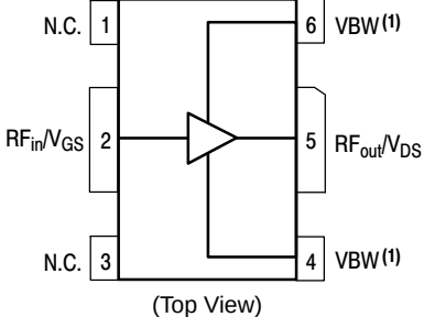
Figure 1. Pin Connections
