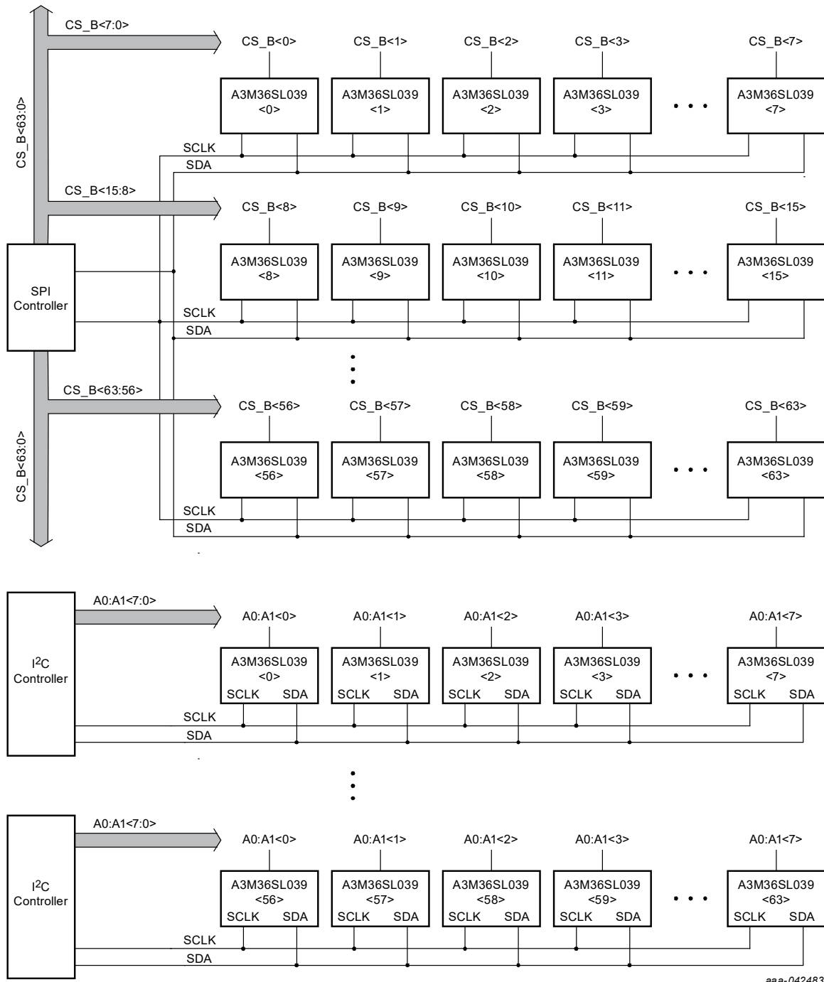
Figure 12. Parallel connectivity of grouping
