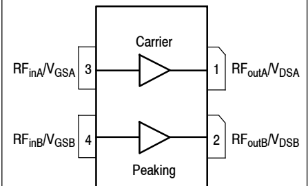
Figure 1. Pin Connections
