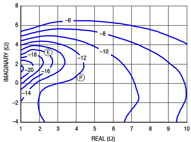
Figure 16. P3dB Load Pull AM/PM Contours (°)
