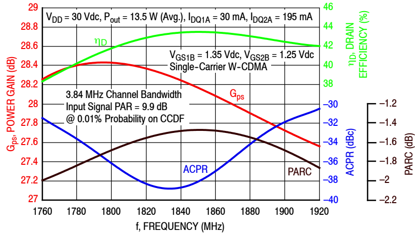
Figure 4. Single-Carrier Output Peak-to-Average Ratio Compression (PARC) Broadband Performance @ P_{out} = 13.5 Watts Avg.
