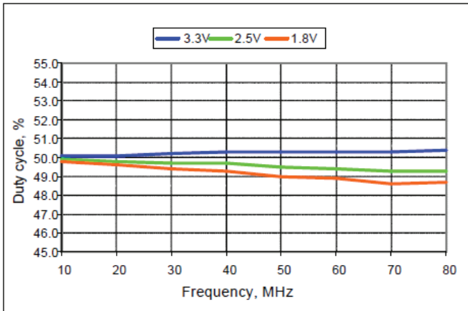
1MHz-80MHz Devices
