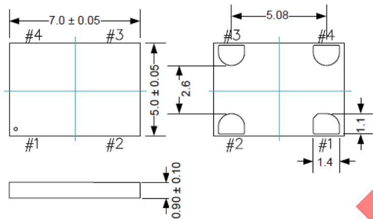
7.0 x 5.0mm Package (Option "V")
