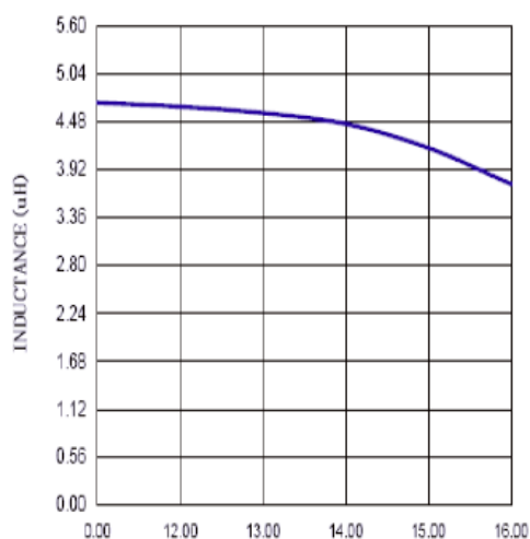
ASPI-1306T-4R7M
