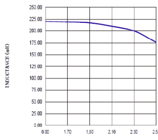
CURRENT (A) ASPI-1306T-221M
