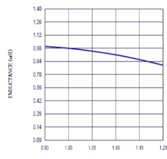
CURRENT (A) ASPI-1306T-102M
