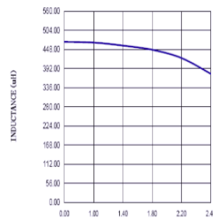
CURRENT (A) ASPI-1306T-471M
