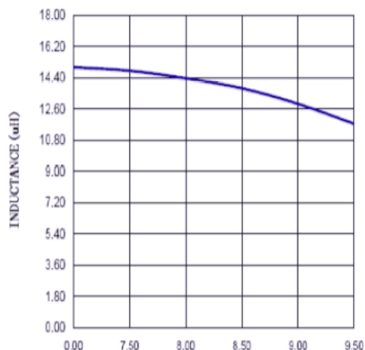
ASPI-1306T-5R6M
