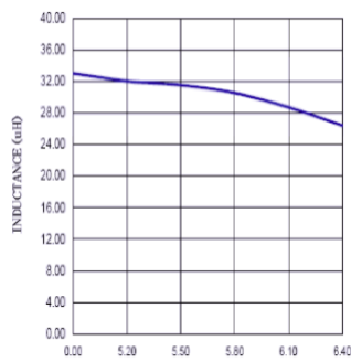
CURRENT (A) ASPI-1306T-330M
