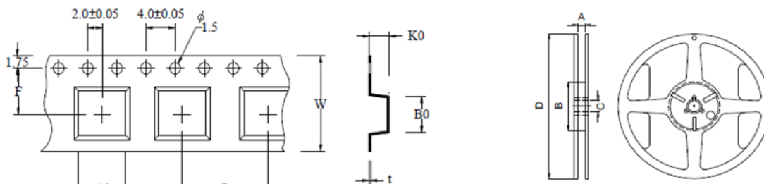
REEL DIMENSION
