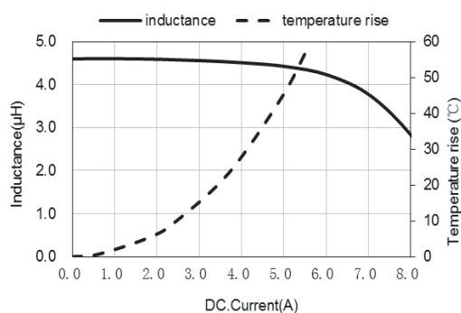
ASPIAIG-S8050-4R7
