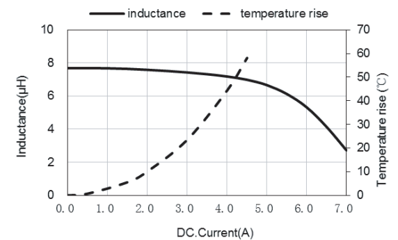
ASPIAIG-S8050-8R2
