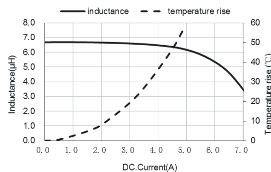
ASPIAIG-S8050-6R8
