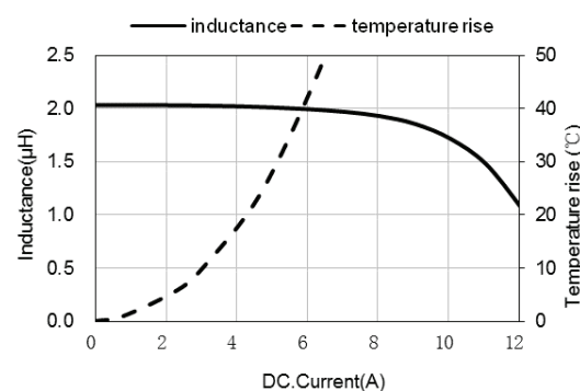
ASPIAIG-S8050-2R2
