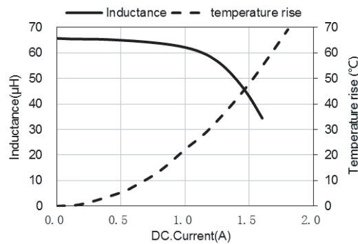
ASPIAIG-S6055-680
