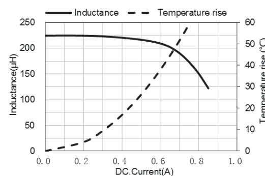
ASPIAIG-S6055-221
