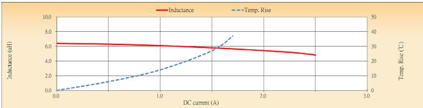
ASPI-M3015-6R8
