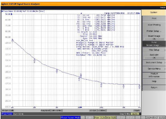
Frequency: 24.576 MHz, VDD: 3.3V
