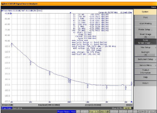
Frequency: 49.152MHz, VDD: 3.3V
