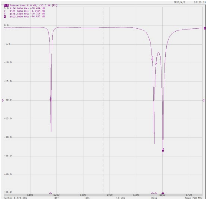
Return Loss
