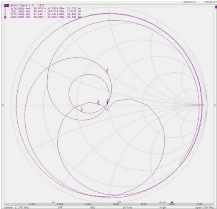
Smith Chart
