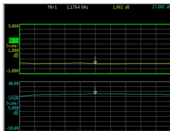
LNA Noise Figure @3.3V
