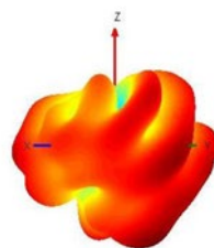
Wi-Fi 2440 MHz
