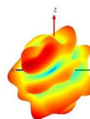
LTE 2690 MHz
