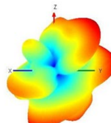
LTE 1850 MHz
