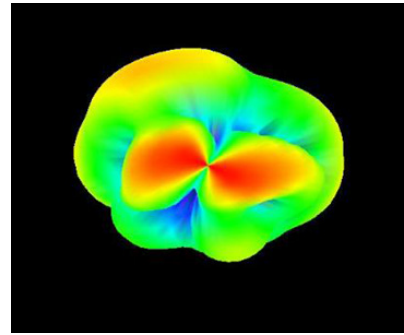
1850 MHz
