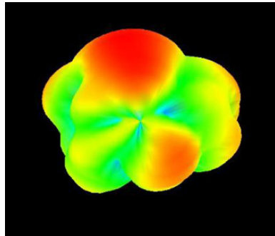
1990 MHz
