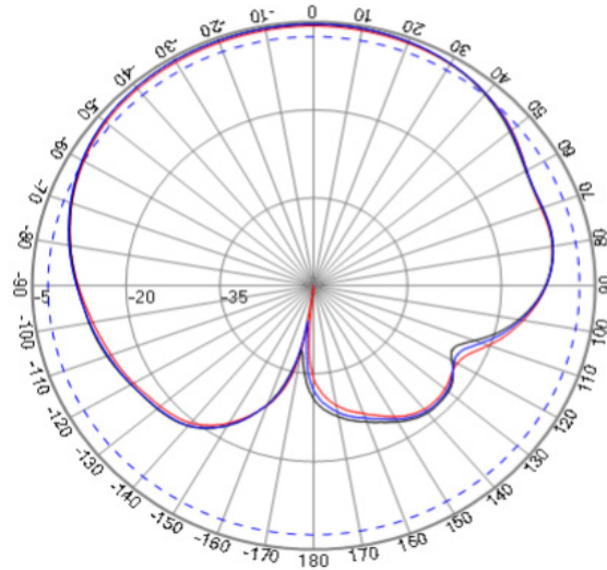
YZ - Plane
