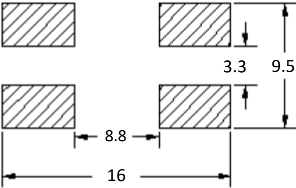
Recommended Layout
