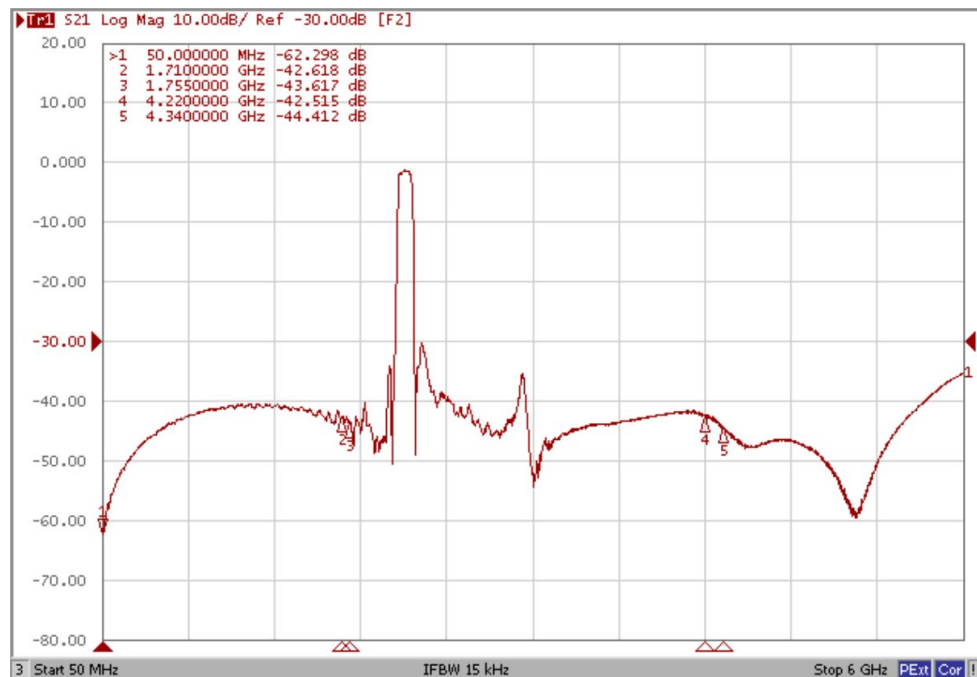
S21 (Broadband)
