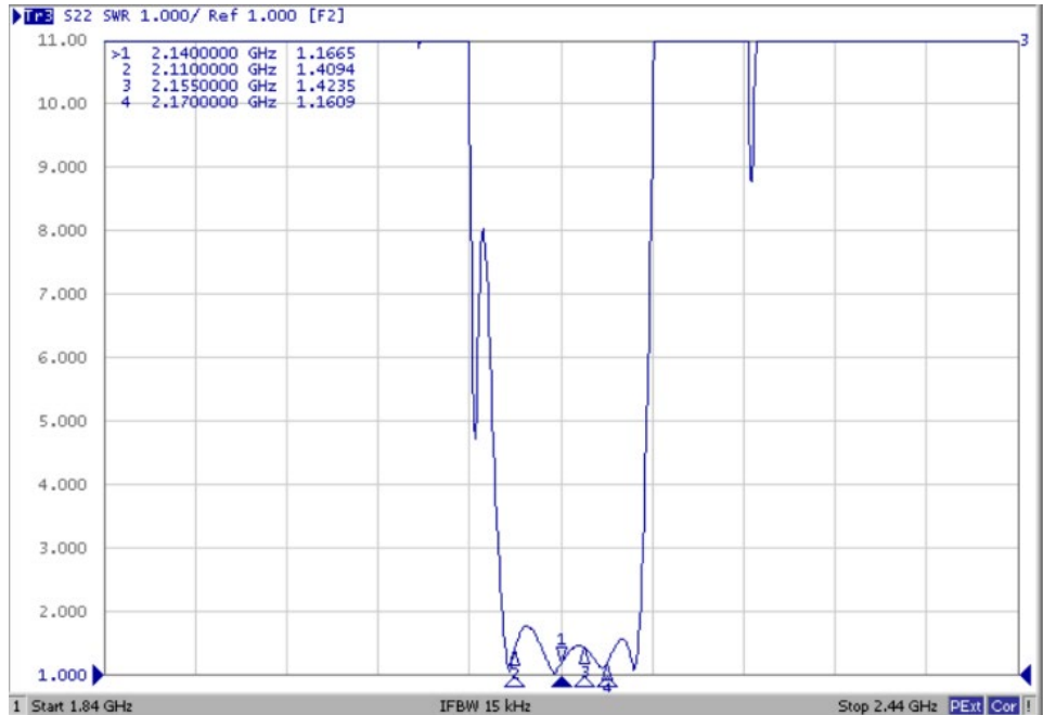
S22 (Narrowband)
