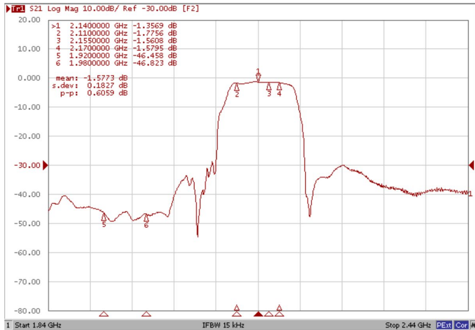
S21 (Broadband)
