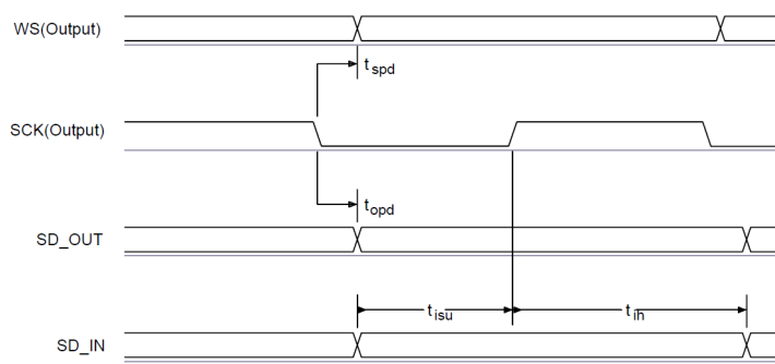
Figure 5. Digital Audio Interface Master Timing
