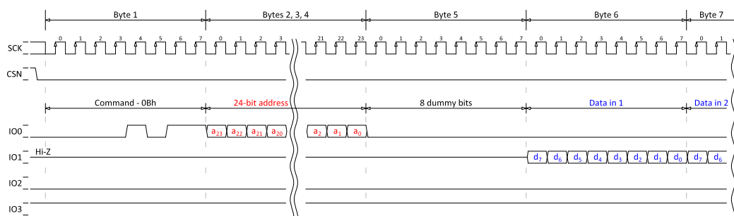
Figure 188: 24-bit FASTREAD, SPI MODE = MODE0
