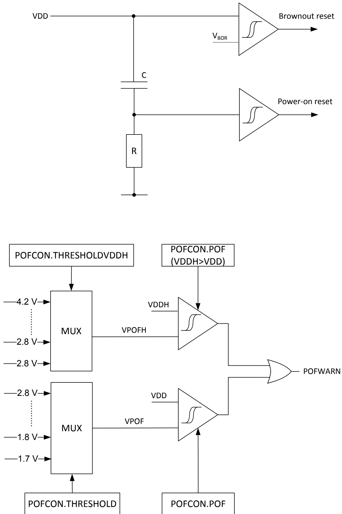
Figure 14: Power supply supervisor
