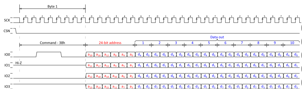
Figure 196: 24-bit PP4IO (quad page program input/output), SPI MODE = MODE0
