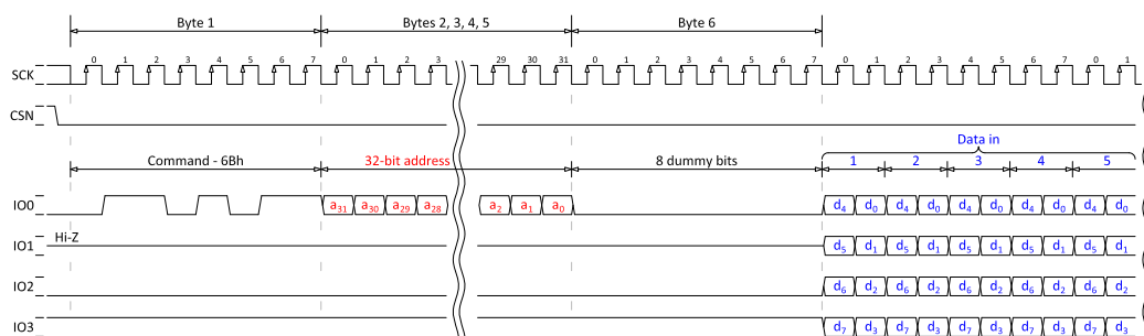
Figure 200: 32-bit READ4O (quad-read output), SPI MODE = MODE0
