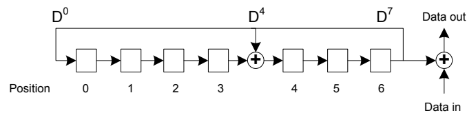
Figure 33: Data whitening and de-whitening
