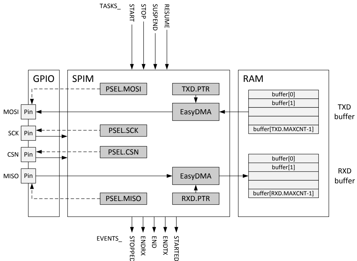
Figure 77: SPIM — SPI master with EasyDMA
