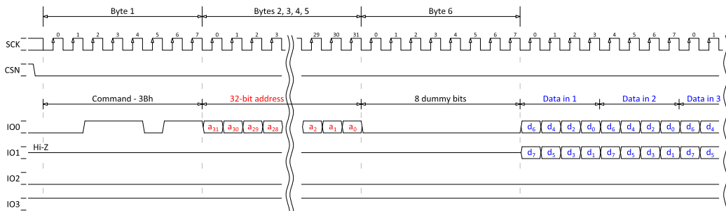
Figure 198: 32-bit READ2O (dual-read output), SPI MODE = MODE0
