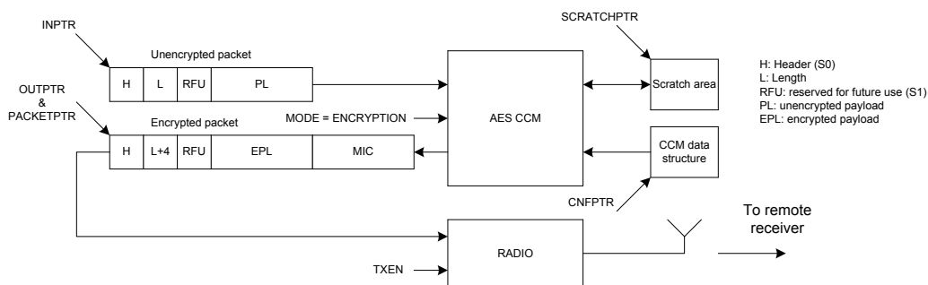
Figure 70: Configuration of on-the-fly encryption
