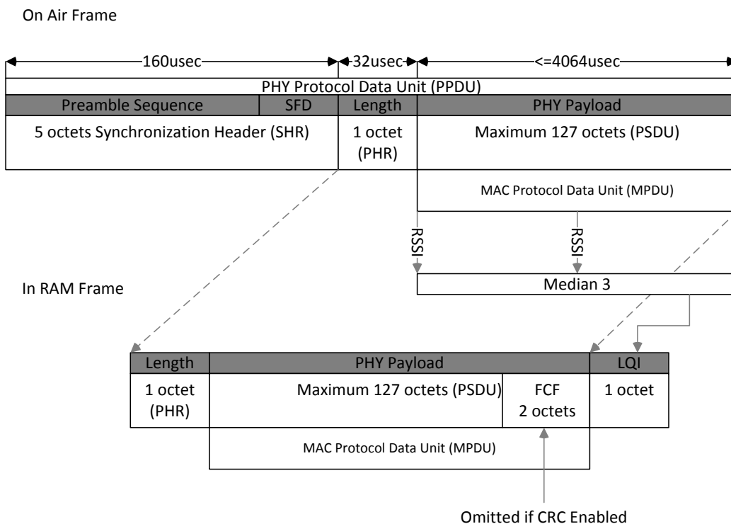
Figure 48: IEEE 802.15.4 Frame In DataRAM
