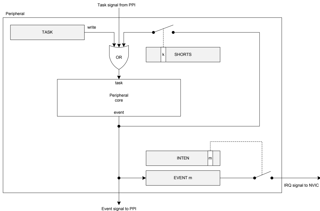
Figure 8: Tasks, events, shortcuts, and interrupts
