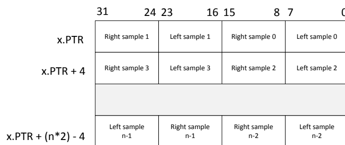
Figure 143: Memory mapping for 8 bit stereo. CONFIG.SWIDTH = 8Bit, CONFIG.CHANNELS = Stereo.
