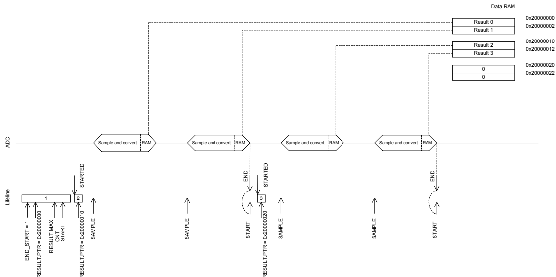
Figure 108: ADC
