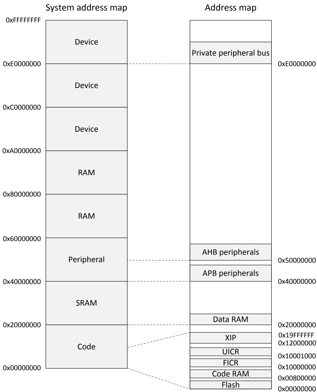
Figure 4: Memory map
