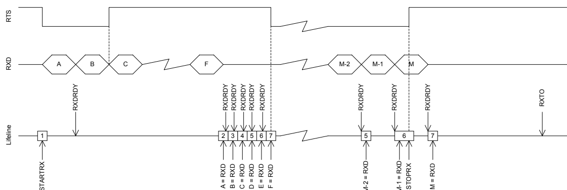
Figure 171: UART reception
