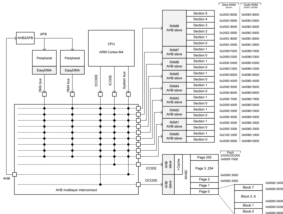
Figure 3: Memory layout
