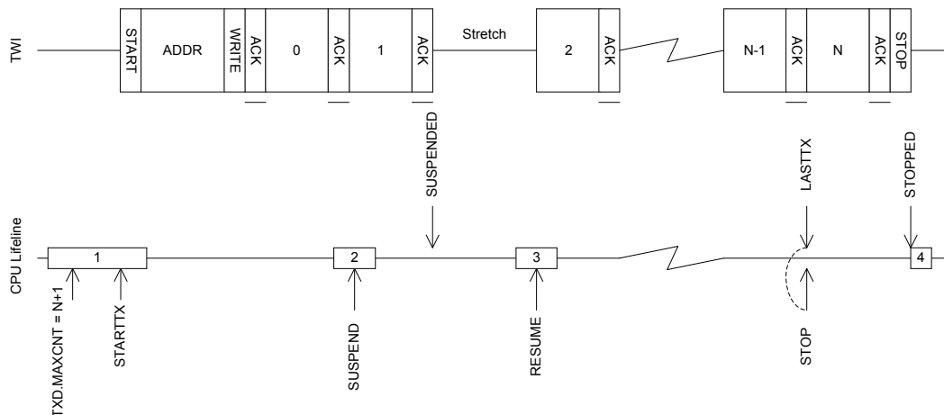
Figure 87: TWI master writing data to a slave
