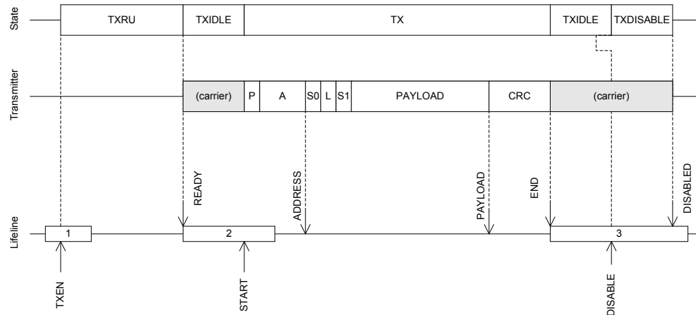
Figure 36: Transmit sequence
