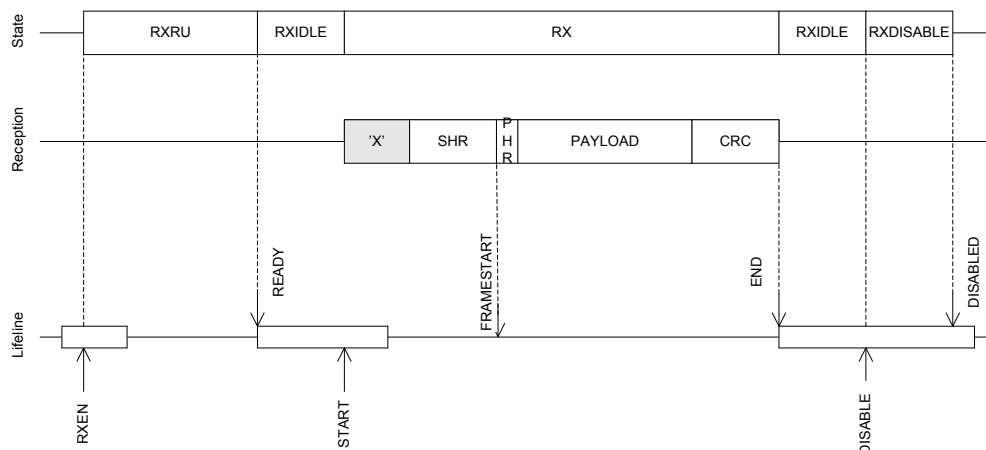
Figure 47: IEEE 802.15.4 Receive Sequence
