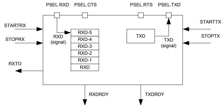
Figure 169: UART configuration
