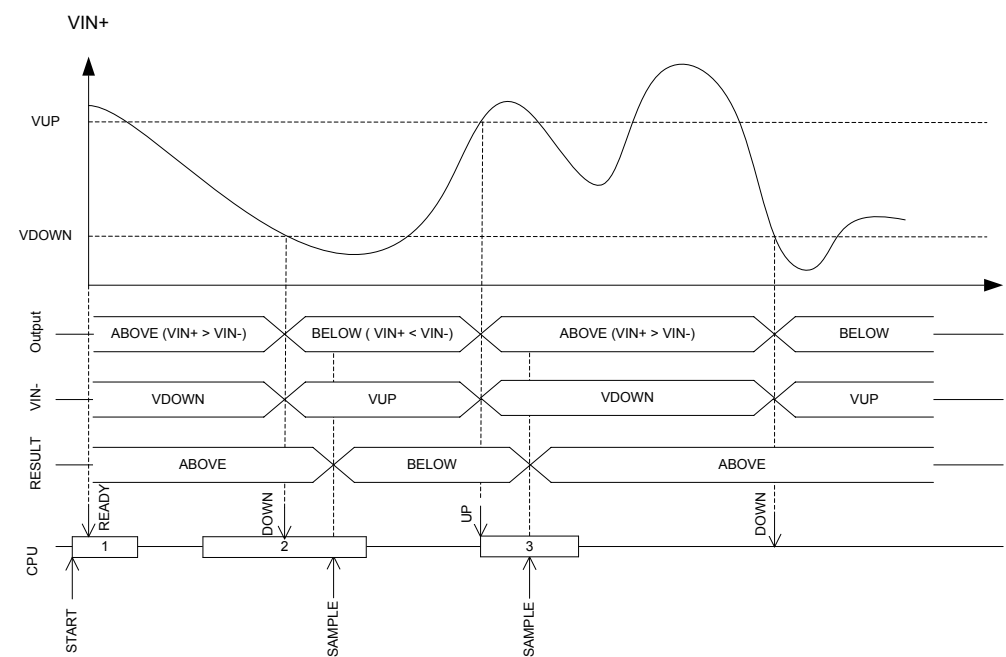
Figure 40: Hysteresis example where VIN+ starts above VUP
