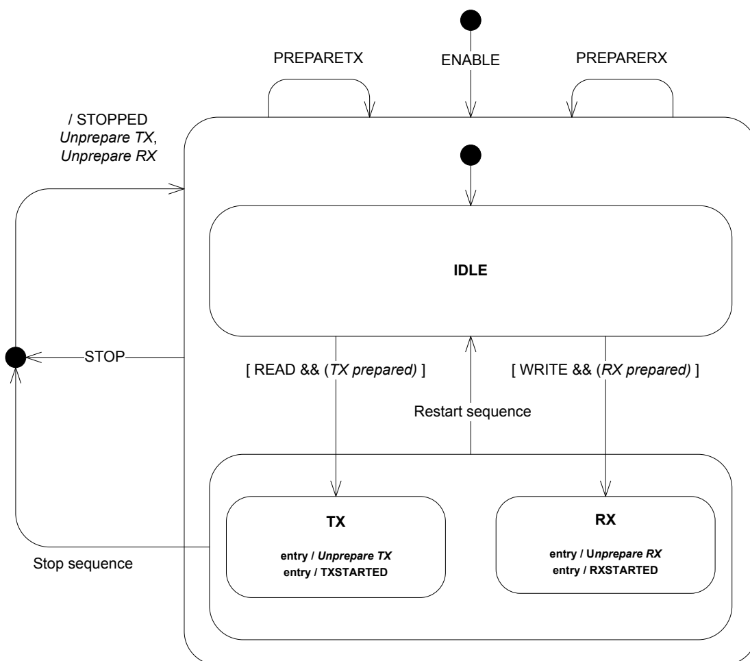
Figure 127: TWI slave state machine
