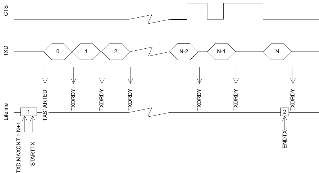
Figure 136: UARTe transmission
