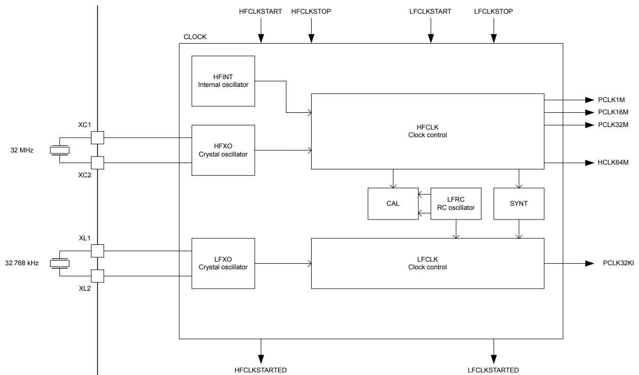
Figure 19: Clock control
