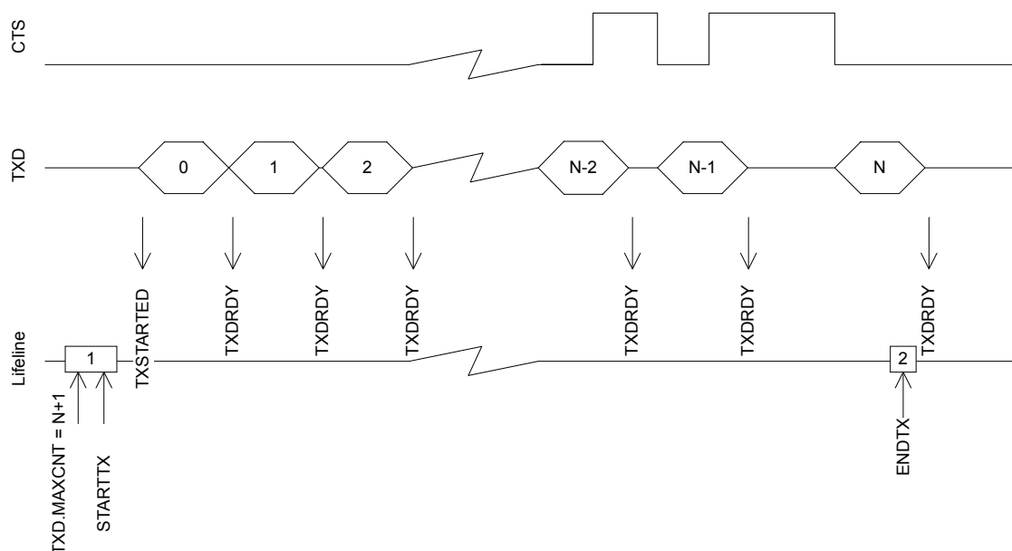
Figure 114: UARTE transmission
