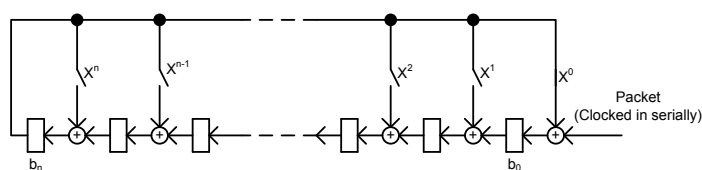
Figure 41: CRC generation of an n bit CRC
