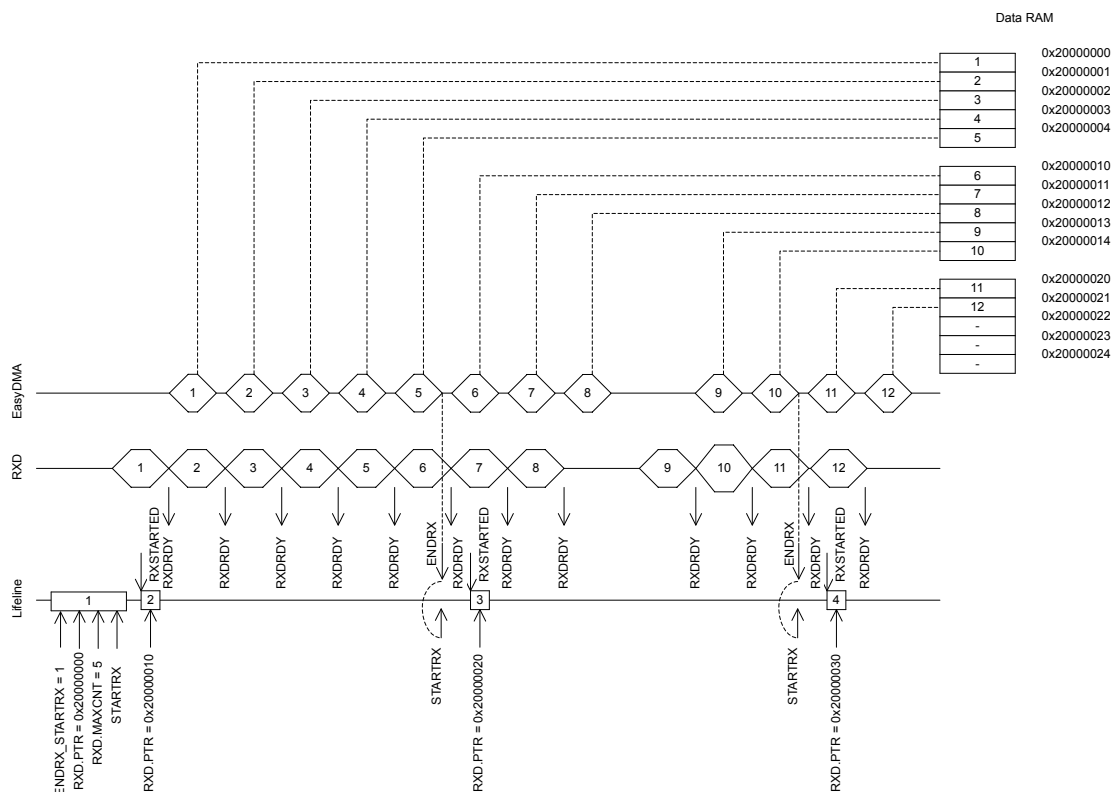
Figure 115: UARTE reception
