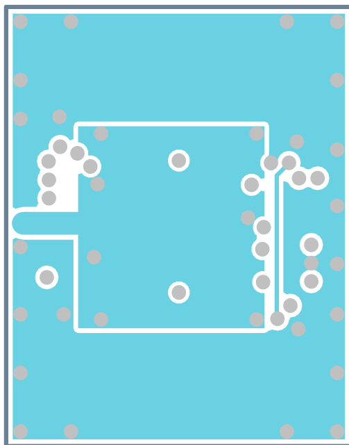
Figure 30: Inner layer 2
