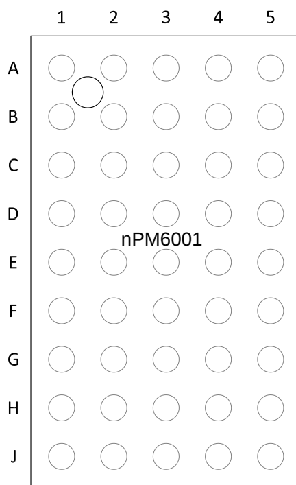
Figure 21: WLCSP ball assignments, top view
