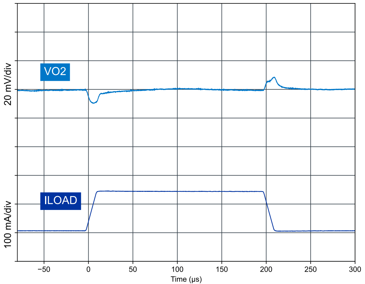
Figure 13: BUCK2 load transient ( V_{IN\_BUCK2} = 3.8\text{ V} , VO2 = 1.2\text{ V} , I_{LOAD} 10 mA - 150 mA)
