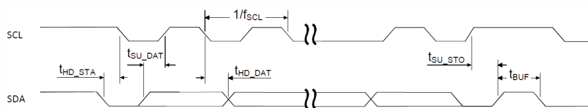
Figure 32: TWI timing diagram
