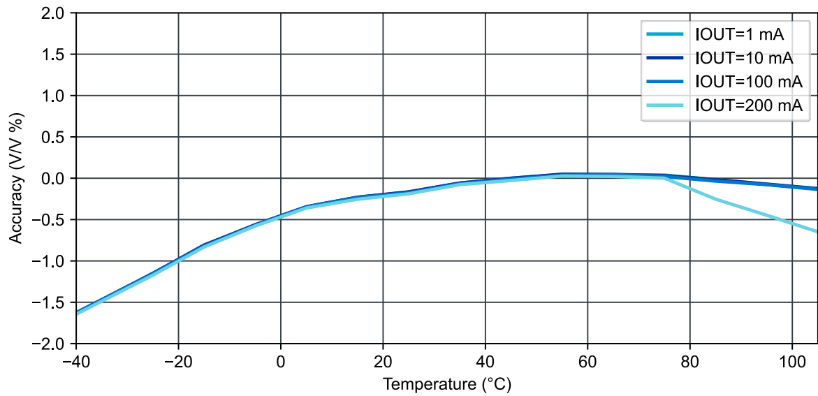
Figure 6: VOO vs. temperature ( V_{IN\_BUCK0} = 3.8\text{ V} , V_{OO} = 3.3\text{ V} )
