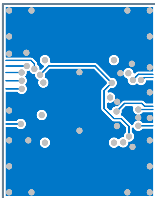
Figure 31: Bottom layer
