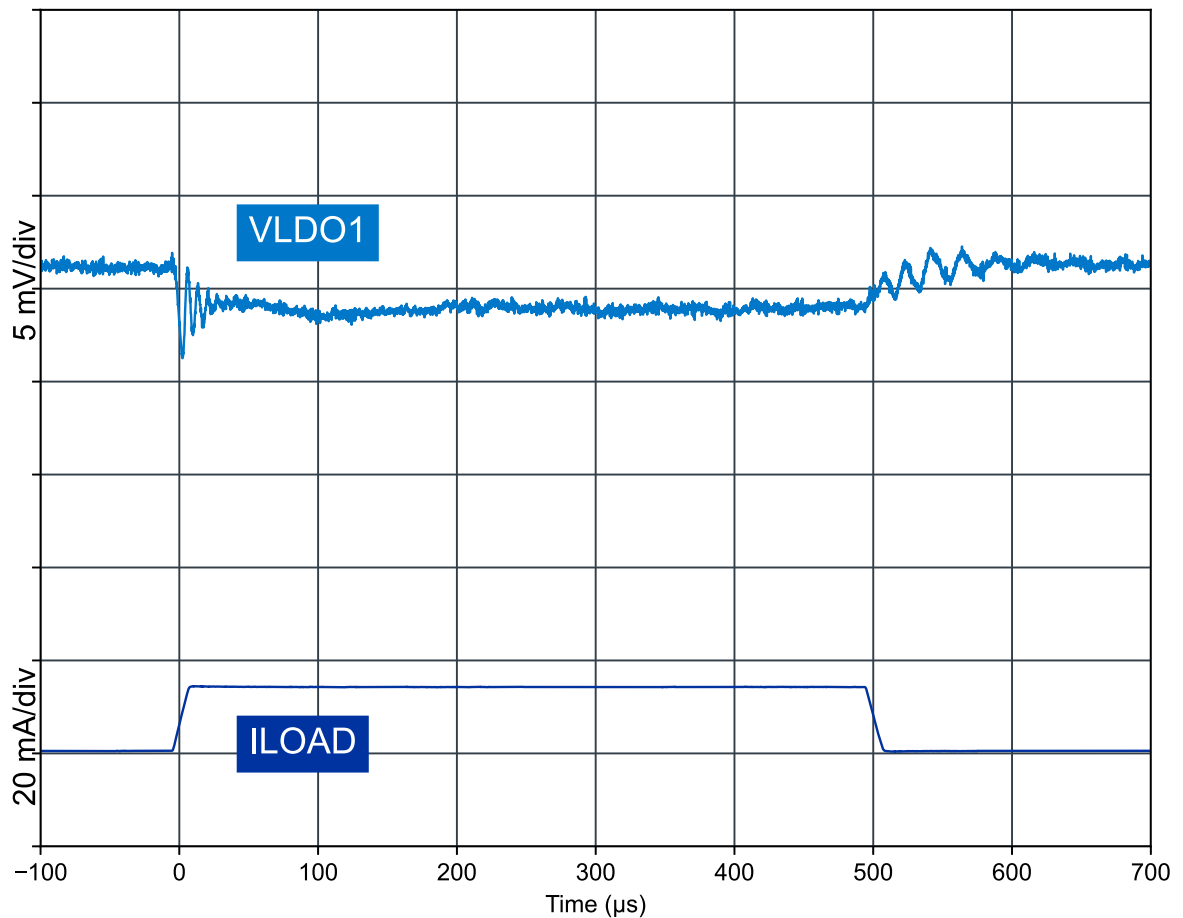
Figure 20: LDO1 load transient ( V_{LDO1} = 1.8\text{ V} , I_{load} 0\text{ mA} - 15\text{ mA} )
