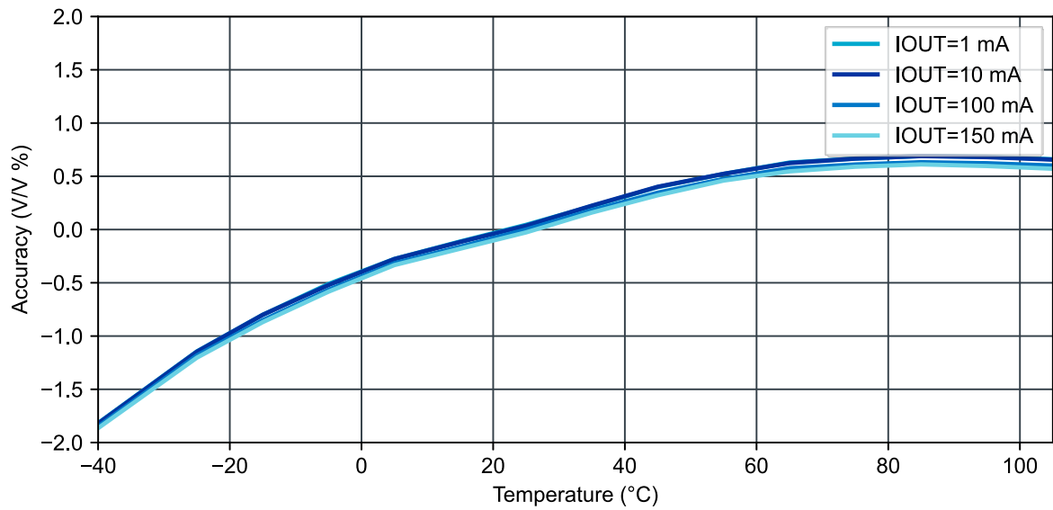
Figure 10: VO1 vs. temperature ( V_{IN\_BUCK1} = 3.8\text{ V} , VO1 = 0.8\text{ V} )
