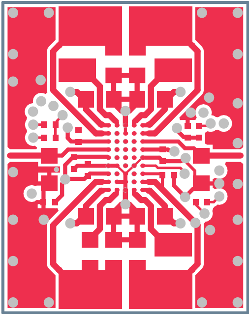
Figure 28: Top layer
