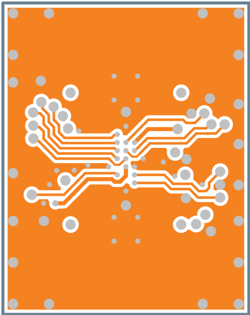
Figure 29: Inner layer 1
