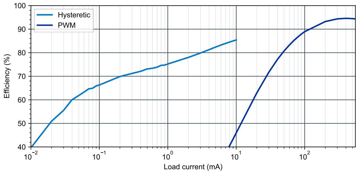
Figure 16: BUCK3 efficiency vs. load current ( V_{IN\_BUCK3} = 3.8\text{ V} , VO3 = 3.3\text{ V} )
