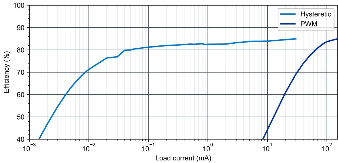
Figure 8: BUCK1 efficiency vs. load current ( V_{IN\_BUCK1} = 3.8\text{ V} , VO1 = 0.8\text{ V} )
