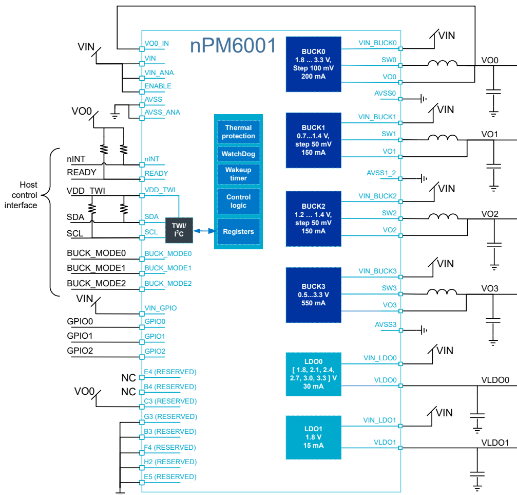
Figure 1: Block diagram
