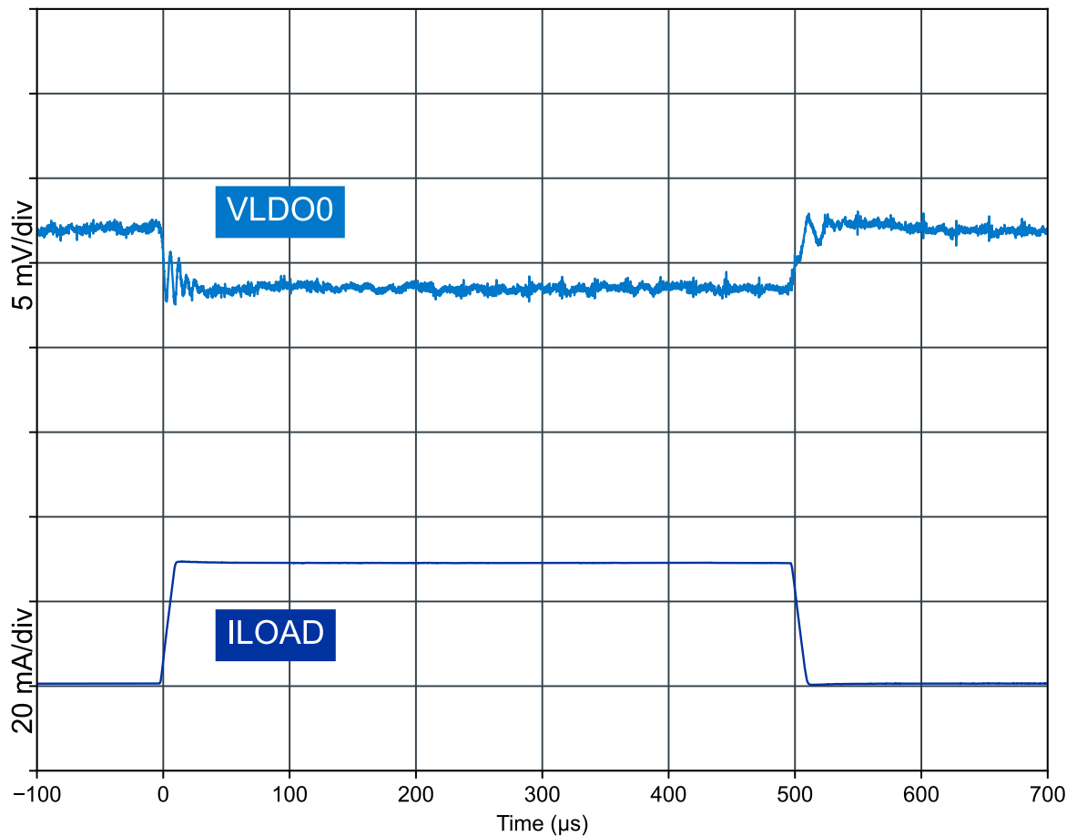
Figure 19: LDO0 load transient (VLDO0 = 3.0 V, I_{load} 0 mA - 30 mA)
