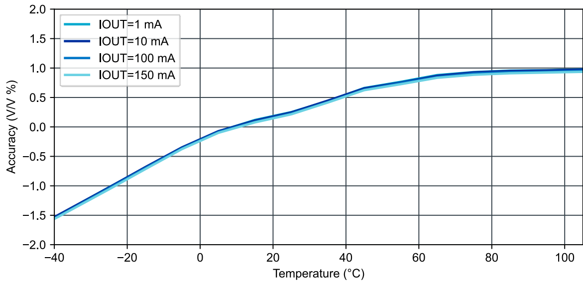
Figure 14: VO2 vs. temperature ( V_{IN\_BUCK2} = 3.8\text{ V} , VO2 = 1.2\text{ V} )
