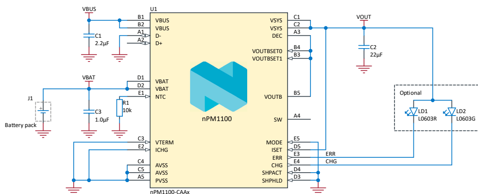
Figure 41: WLCSP schematic
