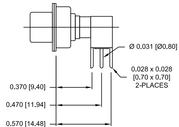
50 OHM COAXIAL CONTACT
