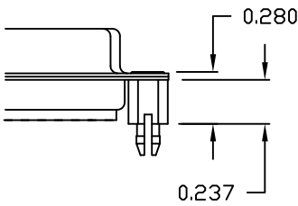
90X ..... 0.237" (BOARD SIDE)
