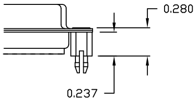
90X ..... 0.237" (BOARD SIDE)
