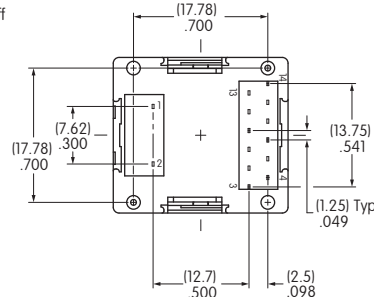
Footprint
