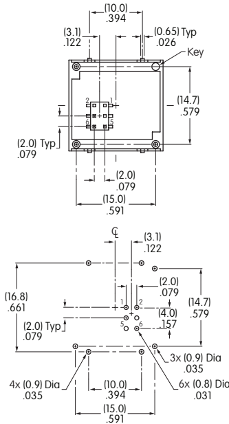
Footprint
