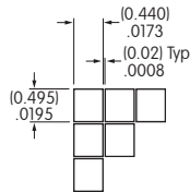
Pixel Detail
