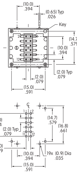
ISO1BBFRGB Super Bright RGB ISO1BBFEF Super Bright Yellow/Green
