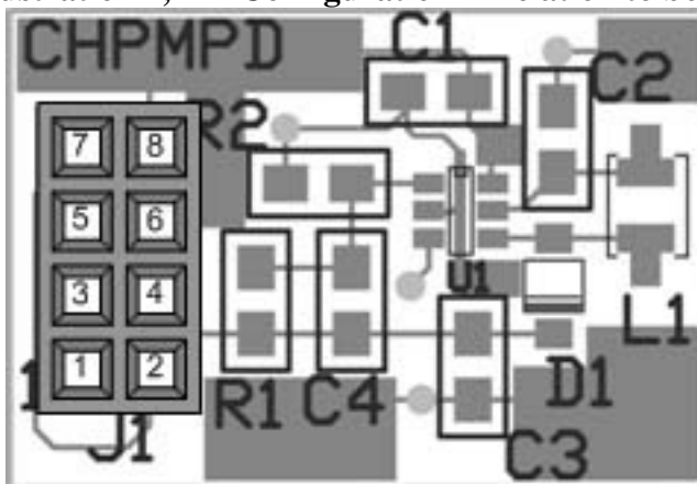
Illustration 1, Pin Configuration in relation to board
