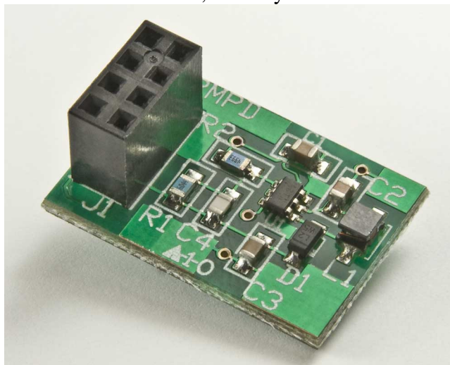
Photo 1, Primary side
