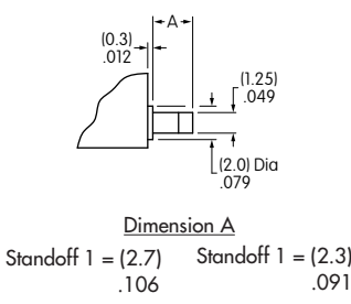
Standoff Detail
