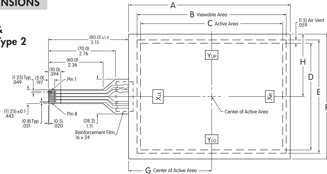
Tail Dimensions for FTAS00-5.7AS-4 FTAS00-6.5AS-4
