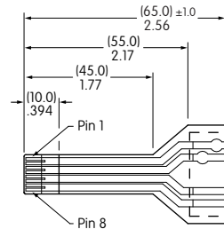
Tail Dimensions for FTAS00-5.7AS-4 FTAS00-6.5AS-4
