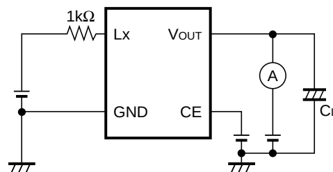
Test Circuit 2
