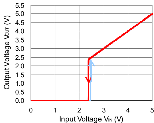
8) Output Voltage vs. Input Voltage
