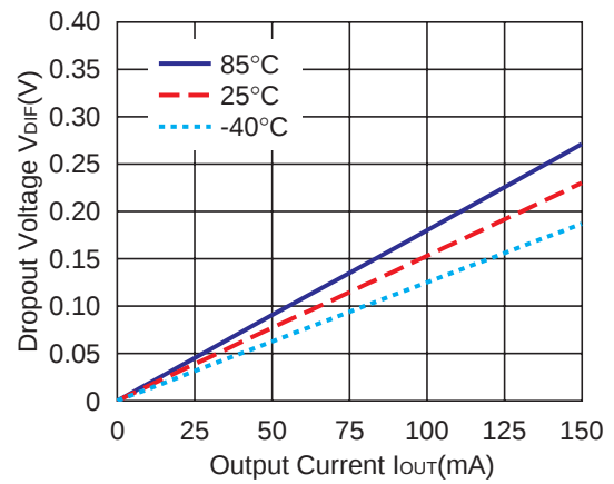
2.0V(VR1/VR2)
