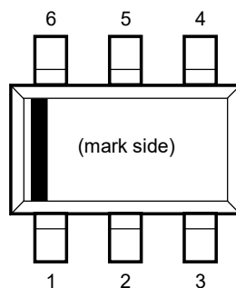
R3121N (SOT-23-6) Pin Configuration
