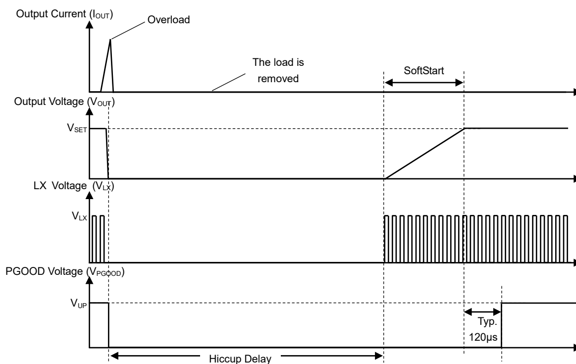
Hiccup-Type Overcurrent Protection Timing Chart
